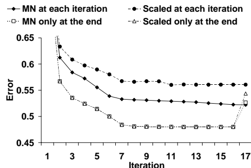
Figure 4: Error per iteration for the four k-medians algorithms on the St. Louis data.
