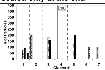
Figure 14: spherical k-means
