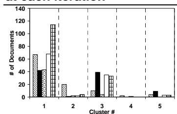
Figure 8: k-medians scaled only at the end
