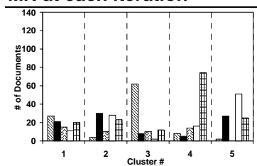
Figure 6: k-medians with MN only at the end
