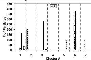
Figure 12: k-medians scaled at each iteration
