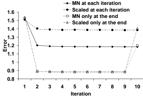
Figure 2: Error per iteration for the four k-medians algorithms on the text data. Note that the algorithms involving scaling consistently perform worse than the algorithms using MN. clusters actually in the data, since this enables an easy scan of the resulting clusters for correctness.
