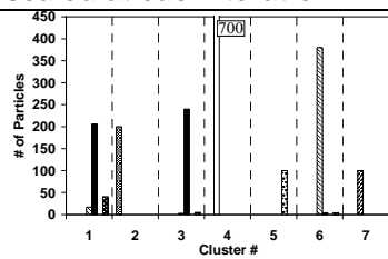
Figure 13: k-medians scaled only at the end
