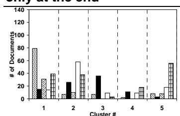
Figure 9: spherical k-means
