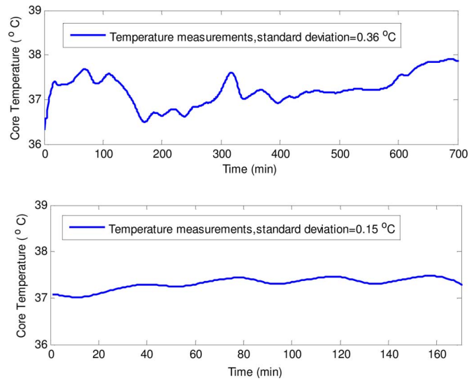
Fig. 3. Temperature profiles for two subjects from the two datasets used in the simulations. Top: Field study, dataset A, Bottom: Laboratory study, dataset B. Note different scales on the x-axis.
