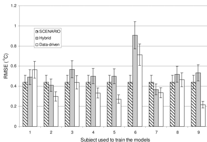
Fig. 9. RMSE for cross-study B-A (simulation S4) predictions. Each bar represents average prediction errors over the eight subjects and four days in dataset A data for AR models (both data-driven and hybrid) trained using the data of the subjects from dataset B indicated on the abscissa. The SCENARIO bars (indicating the same value) represent averaged RMSEs over the four days and all eight subjects in dataset A. The error bounds correspond to one standard deviation. The standard deviation is calculated over all testing subjects and all testing days.
