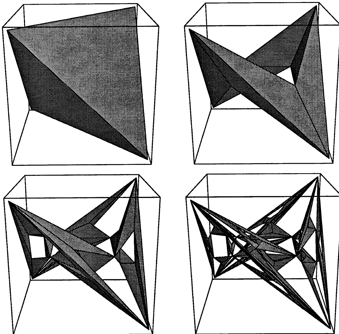
Figure 1: Full-Information Complexes for multi-round Test&Set Protocols
