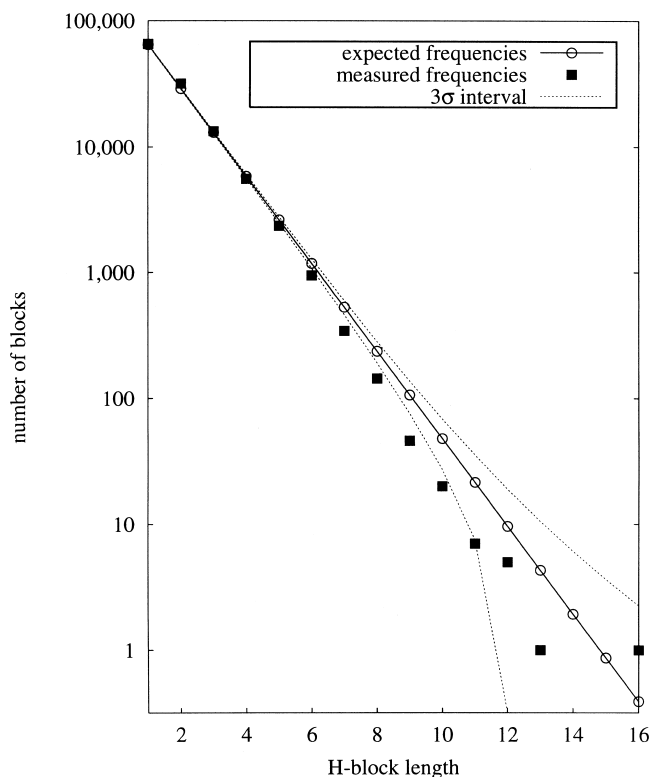
Fig. 1. Semi-log plot of measured values of hydrophobic block length distributions and expected values for non-membrane-associated proteins given the assumption of independence between residues. No measured value is shown for lengths 14 or 15 because no blocks of those lengths were found. Dashed lines show an estimated region of plus or minus three standard deviations about the expectation.
