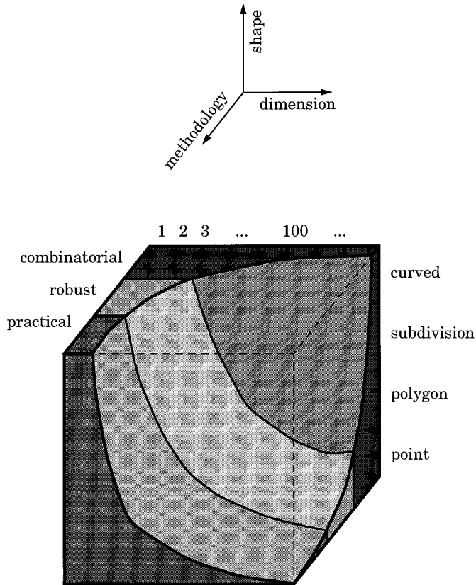
Figure 1. State of the art of computational geometry.
