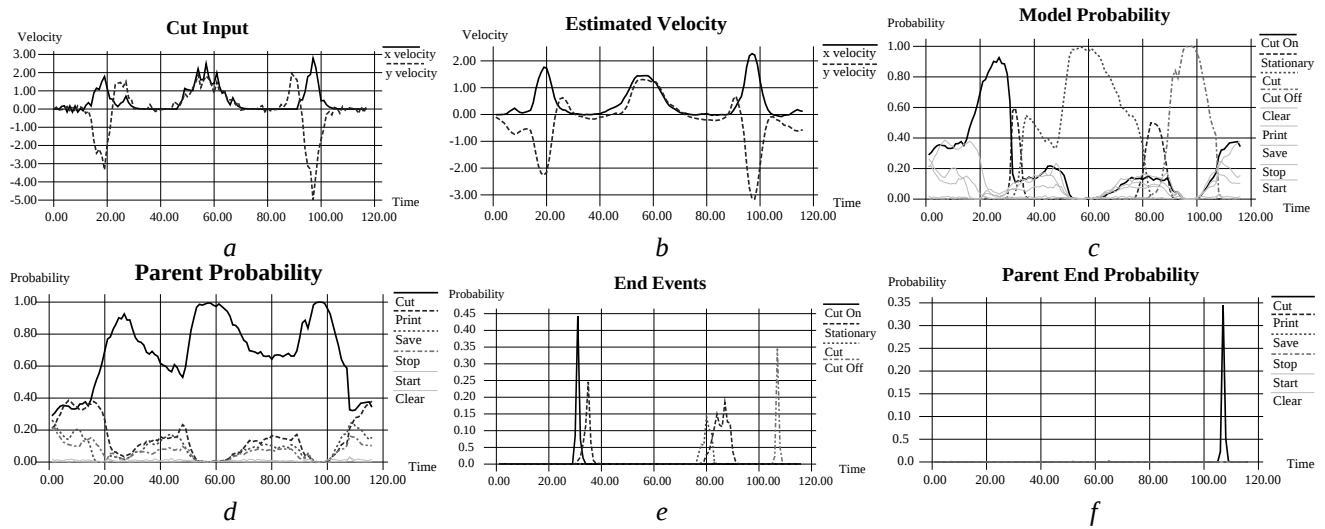
Figure 6: “Cut” gesture. (a), Input horizontal and vertical velocity; (b), Estimated horizontal and vertical velocity; (c), Probability of each event type; (d), Probability of each parent gesture type; (e), Probability that the current state is the completion of an event; (f), Probability that the current state is the completion of a parent.
