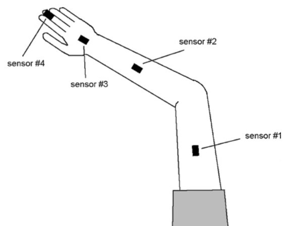
Figure 2. Location of Polhemus FastTrak sensors on the subject's arm.
