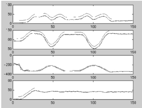
Figure 4. Segmenting using zero-velocity crossings. Variables are plotted along the y -axis against time on the x -axis. The four sub-plots are of the four angles that we analyzed. The curved lines above the movement plots represent individual extracted segments.
