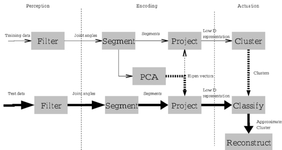
Figure 3. Components of our system. Thin lines represent the flow of data in the training phase. Thick lines represent the flow of data in the testing phase. All dashed lines represent the use of previously computed data. The three layers of the imitation model are shown vertically, as they relate to the specific system components.
