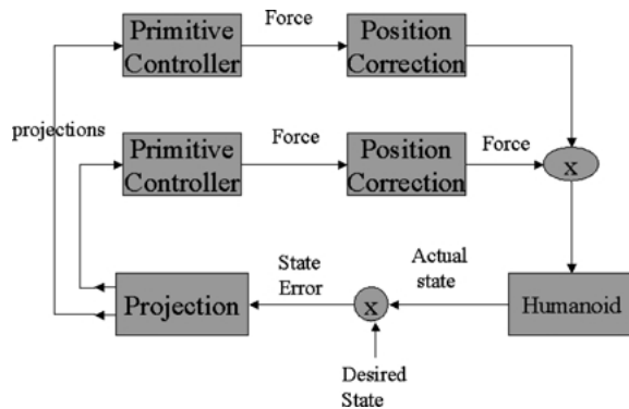
Figure 8. A controller model. The Primitive Controller is an individual controller for each primitive. The Position Correction module corrects for changes in the location of the center of the stroke. The Projection Module projects the errors back onto the eigenmovement space.
