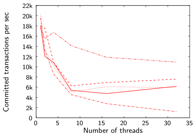
Figure 2: Skiplist application
