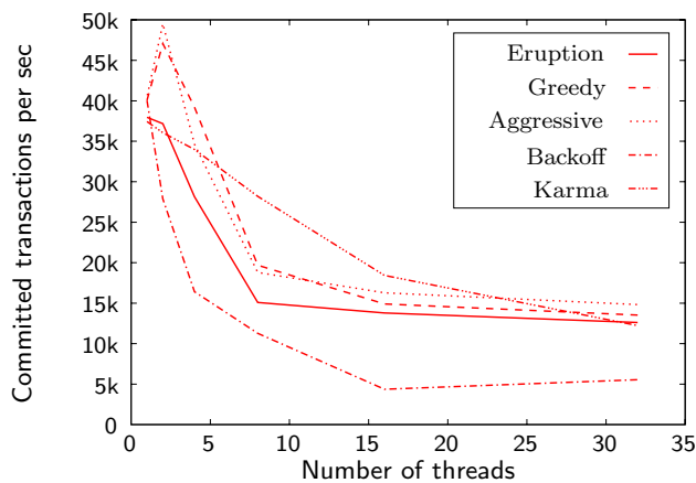
Figure 1: List application
