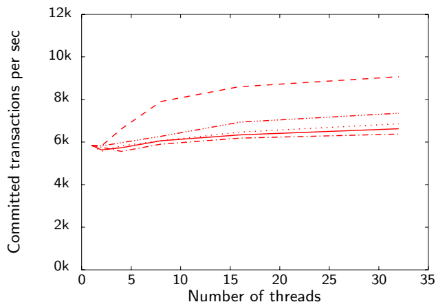
Figure 3: Red-black application (low contention)
