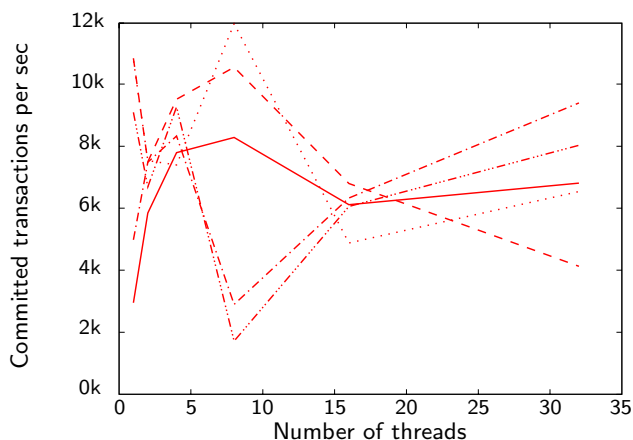
Figure 4: Red-black forest application
