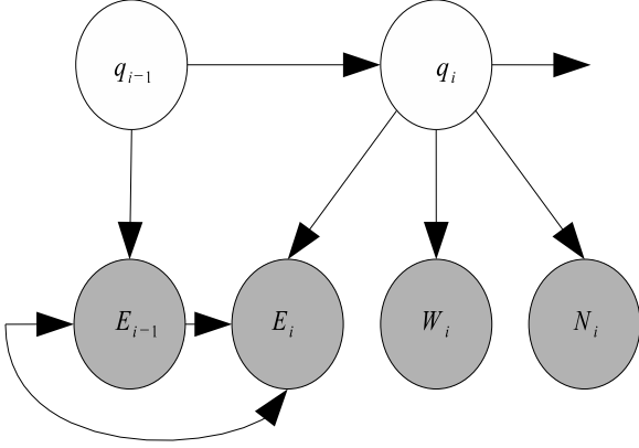
Figure 3: A single time-slice of our HMM.
