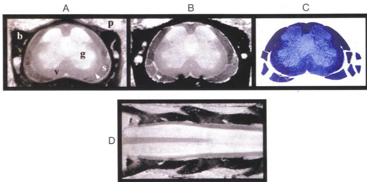
FIG. 1. Images using several imaging modalities. All were acquired in the lumbar region of the same wild-type spinal cord. (A) A volume-rendered transverse image obtained using 3D FLASH with T_2 weighting, TR = 100 ms, TE = 6 ms, and 30\ \mu\text{m} isotropic resolution. (B) A T_2 -weighted I_0 spin-echo image calculated from the 2D diffusion-weighted images with TR = 2000 ms, TE = 17 ms, and 20 \times 20 \times 300\ \mu\text{m} resolution. (C) A 1\text{-}\mu\text{m} -thick epoxy histology section stained with toluidine blue. (D) An alternate view from the same data as in (A) showing several vertebrae in cross section. In (A), various anatomical regions are shown, including trabecula bone (b), ventral column white matter (v), gray matter (g), spinal cord boundary (arrowhead), spinal nerves (s), and PBS (p) inside the capillary tube surrounding the vertebral segment. In (B), the arrowhead points to a hyperintense subarachnoid space outside the spinal cord.
